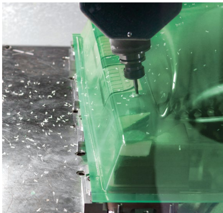
Milling a transparent component in Gibo Plast's Danish factory
